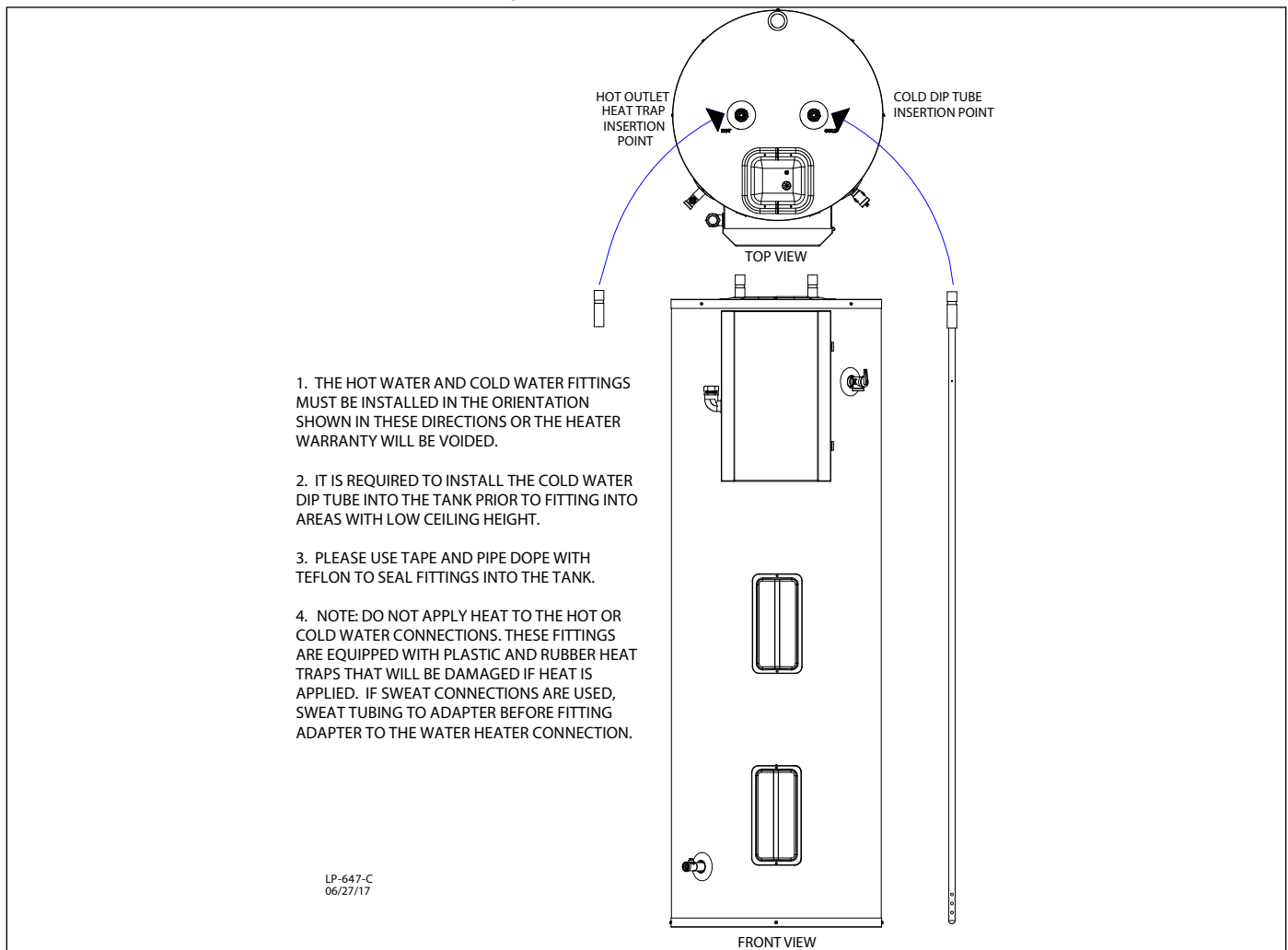
Figure 3 - Installing Cold Inlet and Hot Outlet Fittings
