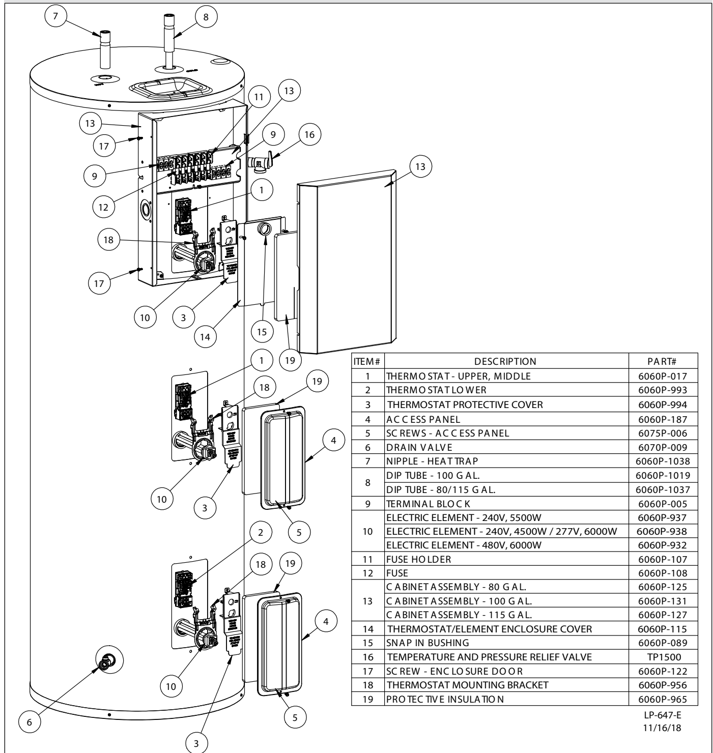
Figure 15 - Replacement Parts
