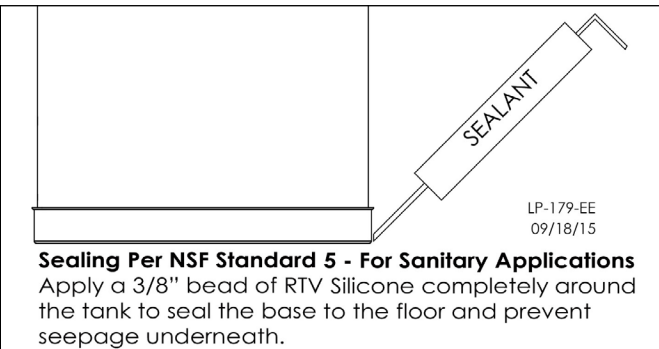
Figure 14 - Sealing the Water Heater for Sanitary Applications
