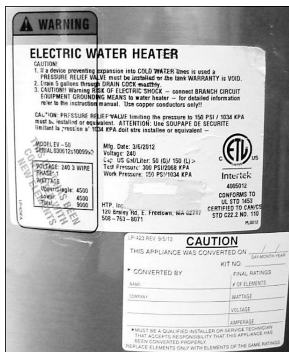
Figure 7 - Example of Conversion Label Replacement
